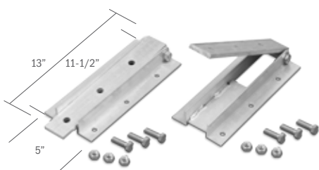
Hinged Sea Wall Brackets R
