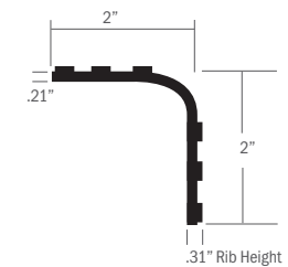
Sectional Mount
