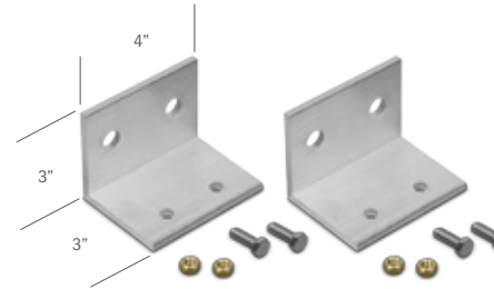
Sectional Sea Wall Brackets S
