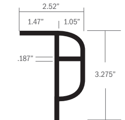
Deck Mount
